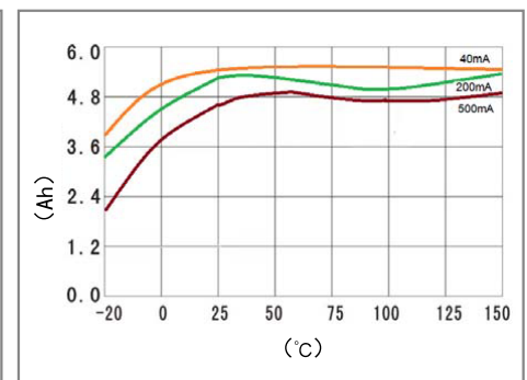
3. CAPACITY VS TEMPERATURE (CUT OFF AT 2.0V)
